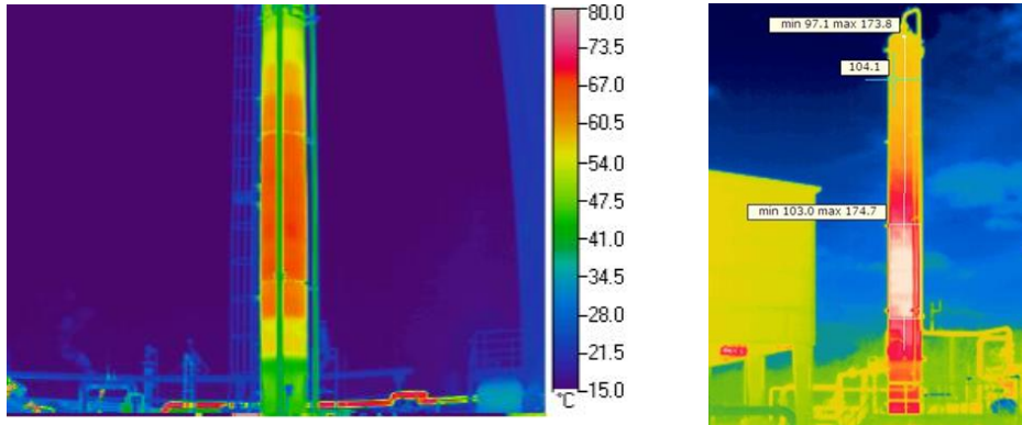
Figure 7. Infrared Scan of Contactor Profiles with Broad Bulge and Bottom Bulge
