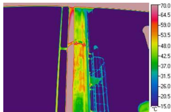
Figure 4. Infrared Camera Photo of Distribution Issue in Packed Tower
