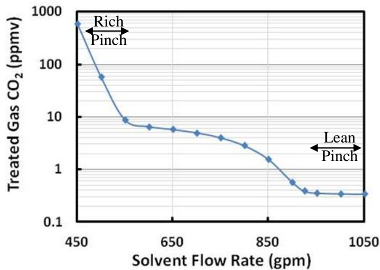
Figure 1. Performance of a Packed LNG Absorber with 0.015 Lean Loading
