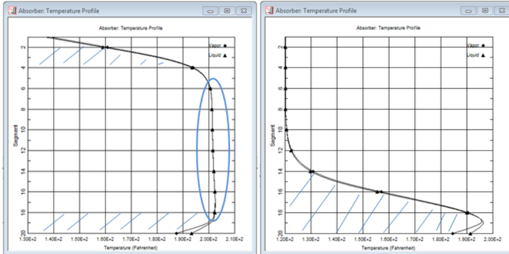
Figure 5 Bulge Pinched and Lean-end Pinched Temperature Profiles
