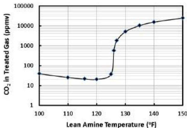
Figure 6: Extreme Sensitivity to Lean Amine Temperature in an LNG Absorber
