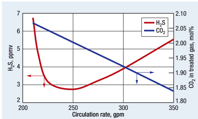
FIG. 4 Processing 330 MMscfd at reduced circulation rate using 20 two-pass trays with 50 wt% generic MDEA.
