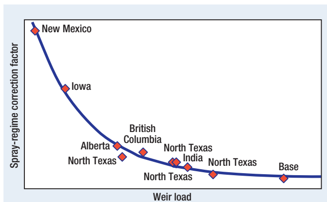
FIG. 1 The correction factor for spray-regime operation varies with weir liquid load.
