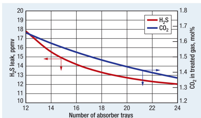
FIG. 2 Adding trays does not meet the treating specification with MDEA at design rates.
