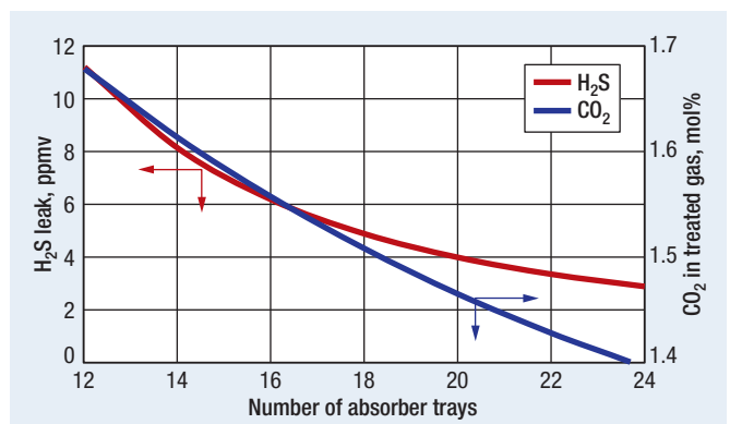
FIG. 3 The use of a stripping promoter meets treat but removes too much CO 2 .
