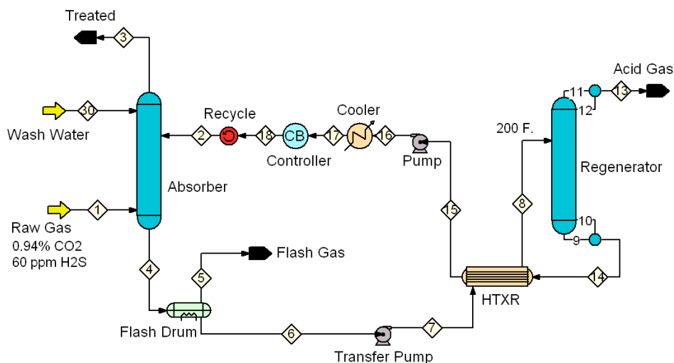
Figure 4 PFD for Case Study 1
