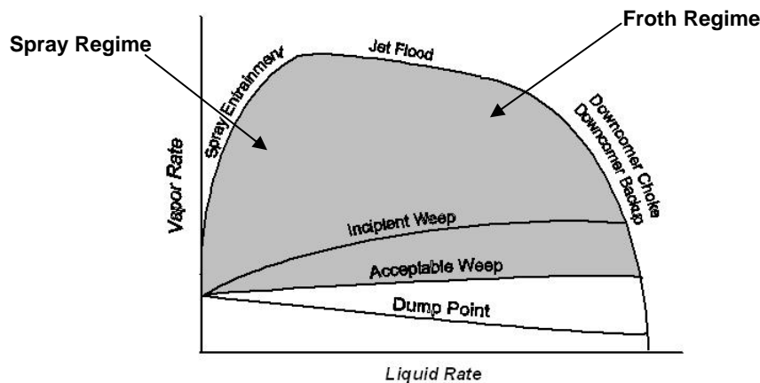
Figure 1 Tray Operating Diagram (adapted from Kister, 1992, p. 269)
