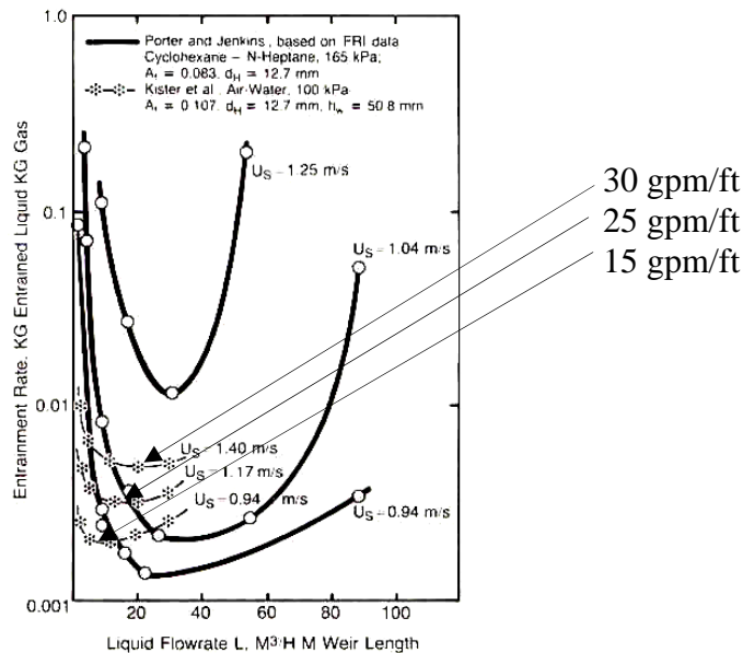
Figure 3 Dependence of Entrainment Rate on Weir Load at Various Gas Rates for Cyclohexane – n-Heptane and Air–Water (Kister & Haas, 1987)
